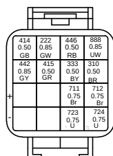
TO ENGINE ROOM HARNESS ( 1-R )
