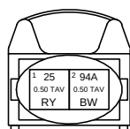
PURGE VALVE (6-E)
