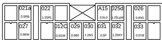
TO ENGINE ROOM ( 4 ) ( 11-I)
