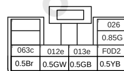
Dashboard key 2 (27-I)
