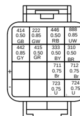
TO ENGINE ROOM HARNESS ( 1-R)
