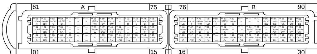
ECU Connector , FRONT VIEW (1-E)
