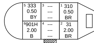
FUEL TANK ( 5-RLD)
