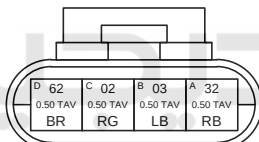
STEPPER MOTOR (9-E)
