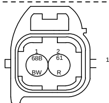
IGNITION COIL CYL 2,3 (13-E)
