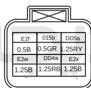
Right headlight set 14-M
