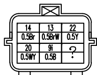
Left front door lock main motor (13-LD)
