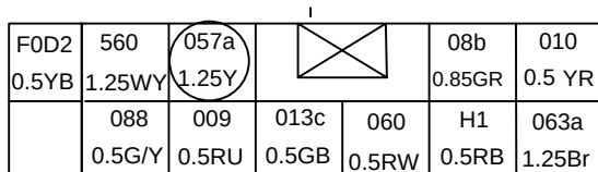
TO ENGINE ROOM (2) (34-I)
