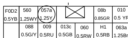
TO ENGINE ROOM ( 2 ) ( 34-I)
