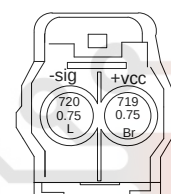
FR WHEEL SENSOR (2-M)
