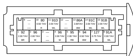
DUAL RELAY (2-E)
